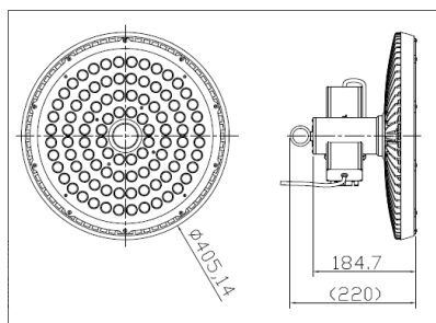
Maße in mm - Ø 405,14
